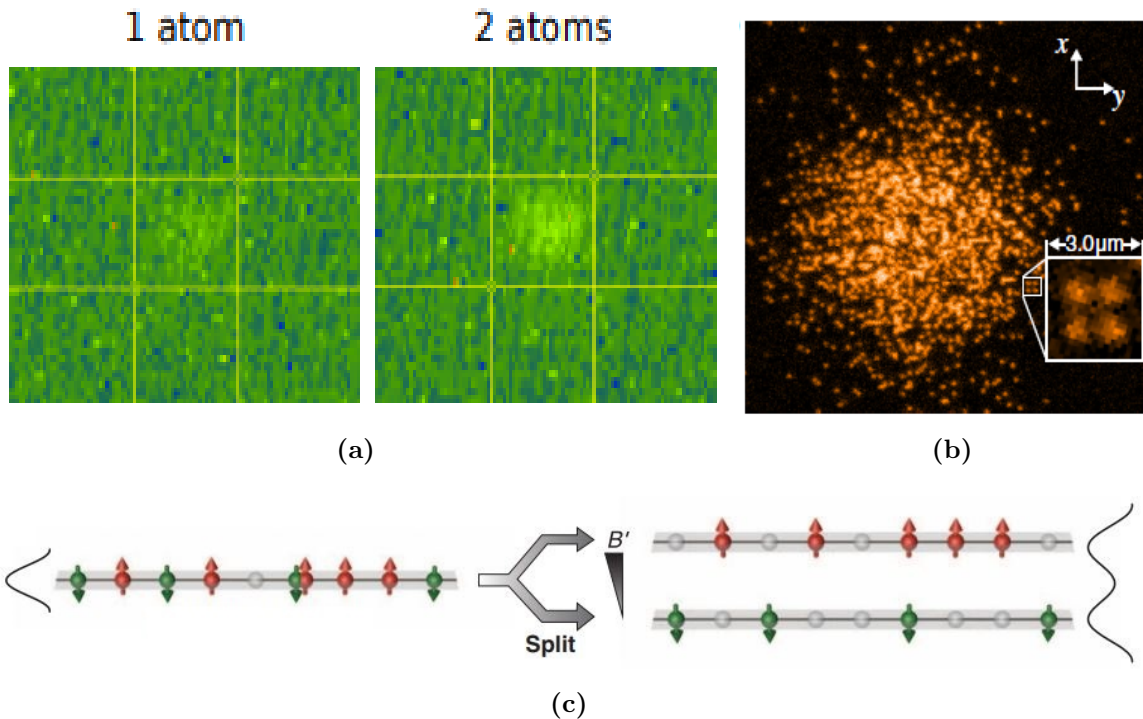
Figure 9 – Single atom detection. (a) A signal from a single atom and two atoms of ^6\text{Li} by using a 3D MOT. This picture was adopted from [29]. In this measurement the photon was collected by lens with \text{NA}=0.17 and exposure time is 0.5 sec. (b) A signal from a single ^{40}\text{K} atom in lattice with high resolution using a Raman sideband cooling technique. In this measurement, the signal per atom is \sim 1000 \frac{\text{photon}}{\text{atom}\cdot\text{sec}} was collected by high NA objective and the exposure time is 1sec. This picture was adopted from [8]. (c) Schematic of the spin-resolved imaging. Each site was split independently into a double-well potential by applying a magnetic field gradient. This picture was adopted from [6].
