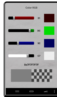
Figure 5: RGB photo
