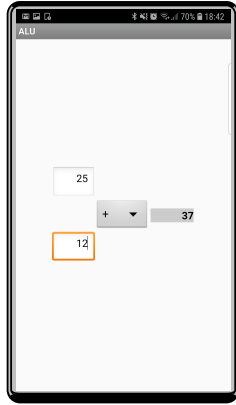
Figure 3: ALU simulator
