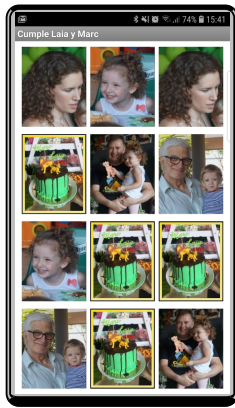
Figure 6: Memory game
