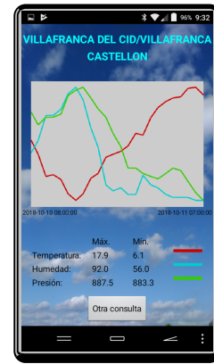
Figure 7: Weather app
