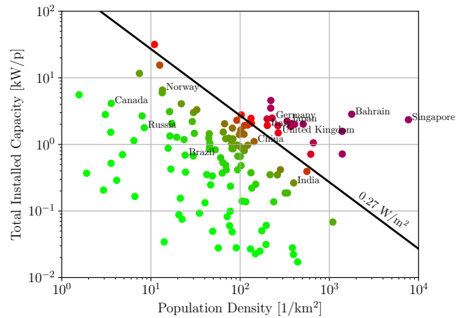
Figure 5: The installed electricity production capacity and population density for 131 countries worldwide (2015 data). The black trend line represents Germany's 2018 b_c = 0.27 \text{ W/m}^2 value.
