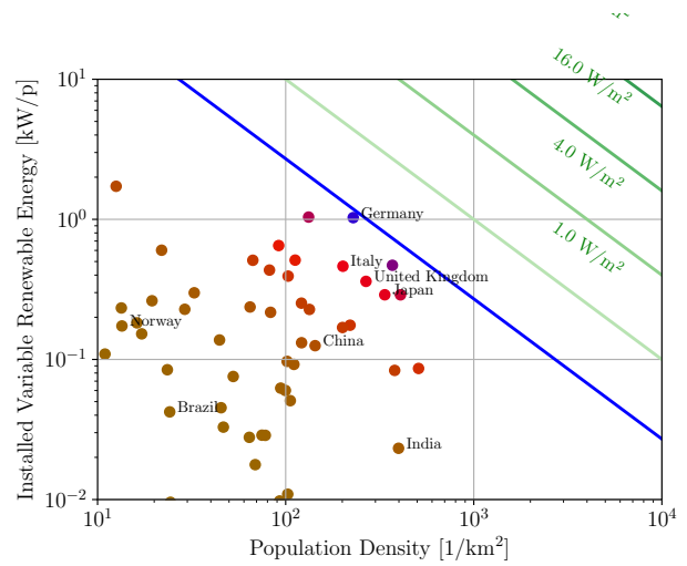
Figure 4: Installed VRE and population density for 131 countries worldwide (2015 data) [34]. The blue trend line represents Germany's (2018) 0.27 \text{ W/m}^2 fit. The green lines represent theoretical solar and wind density calculated theoretical limits of 1.0, 4.0, 16.0 \text{ W/m}^2 .
