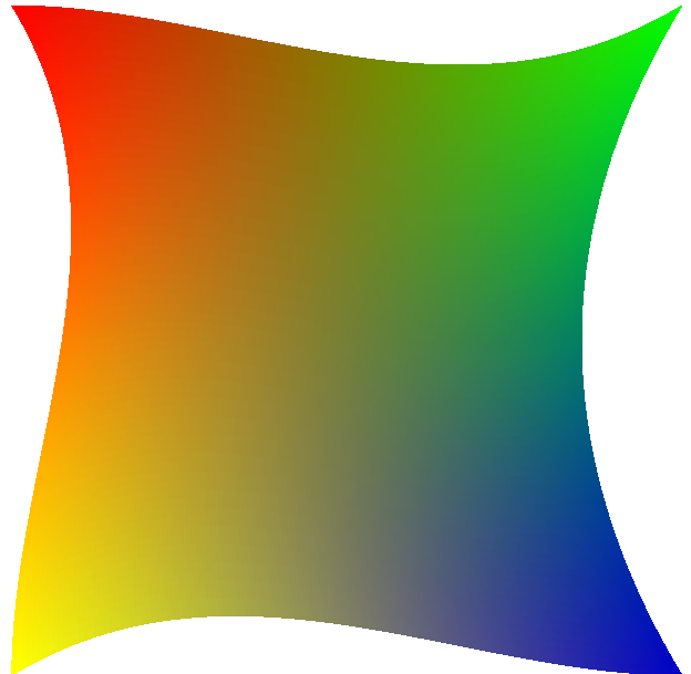
CoonsPatchMesh()
